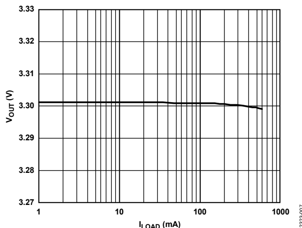
Figure 6. Output Voltage ( V_{OUT} ) vs. Load Current ( I_{LOAD} )
