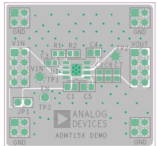
Figure 2. ADM7154RD-1.8EVALZ LFCSP Evaluation Board
