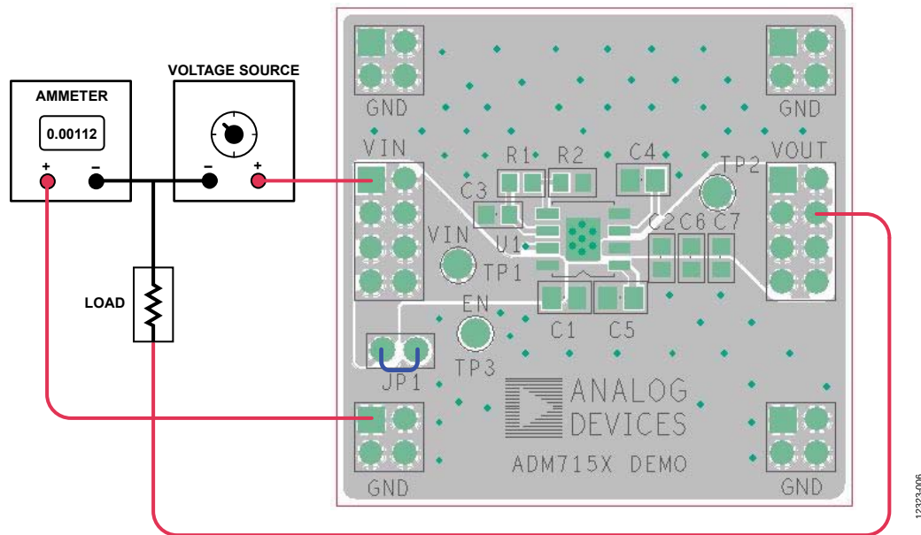
Figure 9. Ground Current Measurement, SOIC
