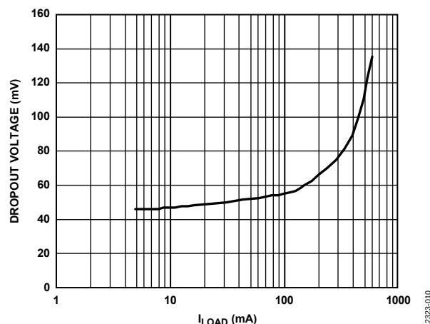
Figure 7. Dropout Voltage vs. Load Current ( I_{LOAD} )
