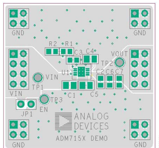
Figure 1. ADM7154CP-3.3EVALZ and ADM7155CP-02-EVALZ LFCSP Evaluation Board
