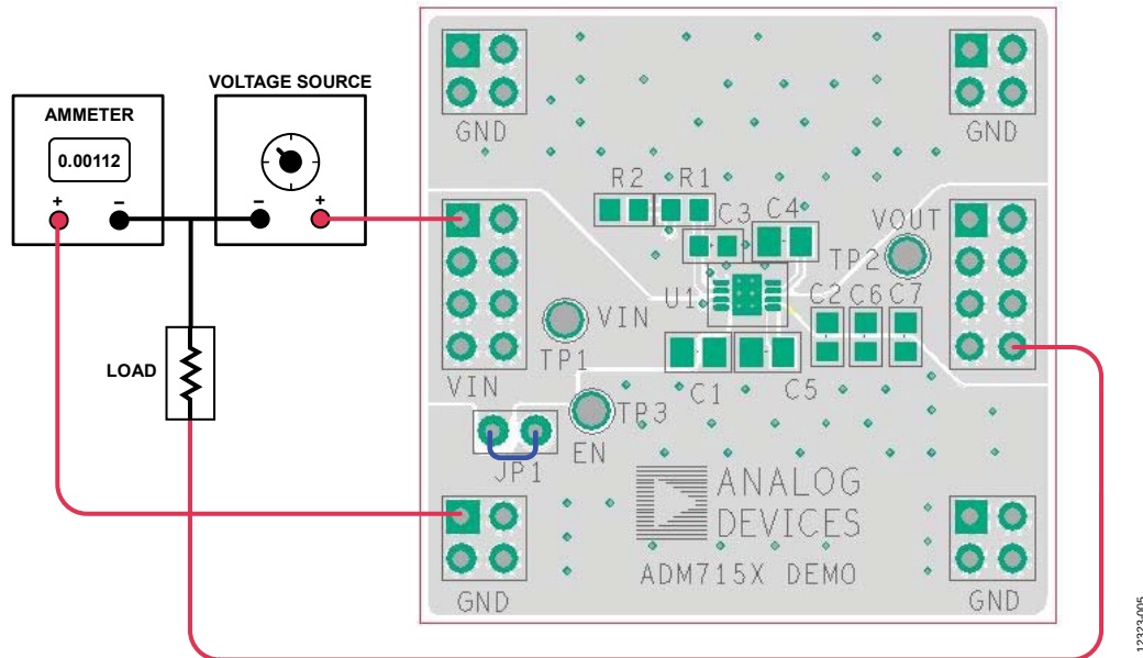
Figure 8. Ground Current Measurement, LFCSP
