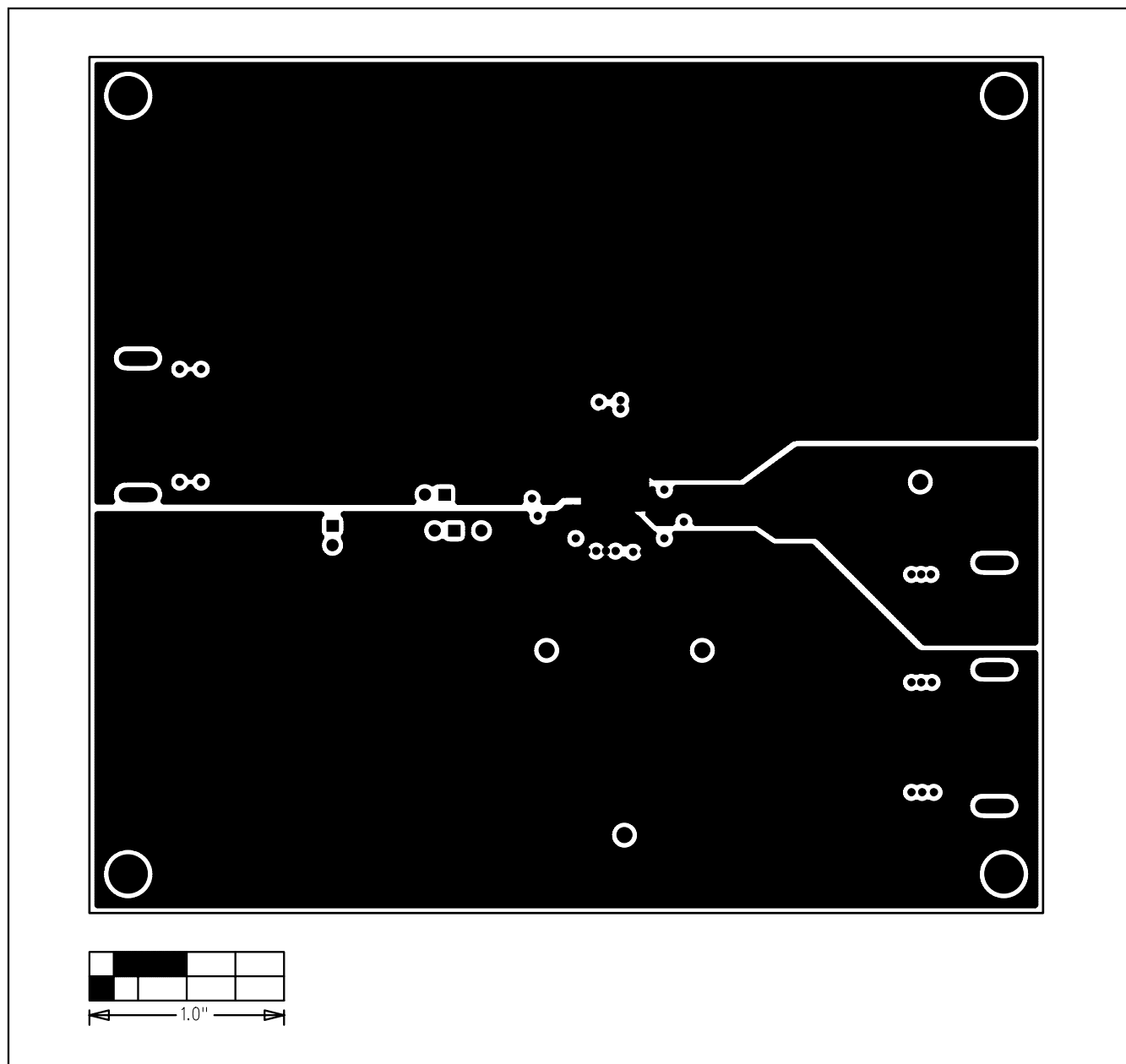
Figure 7. MAX5891/MAX5890/MAX5889 EV Kit PCB Layout—Ground Planes (Layer 2)
