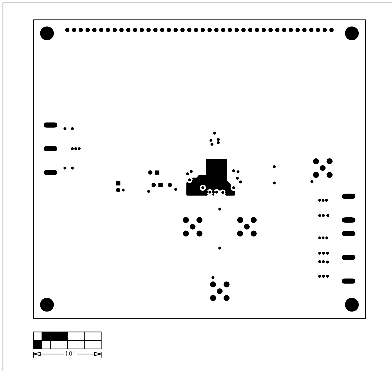
Figure 9. MAX5891/MAX5890/MAX5889 EV Kit PCB Layout—Solder Side (Layer 4)
