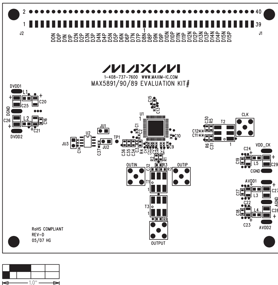
Figure 5. MAX5891/MAX5890/MAX5889 EV Kit Component Placement Guide—Component Side
