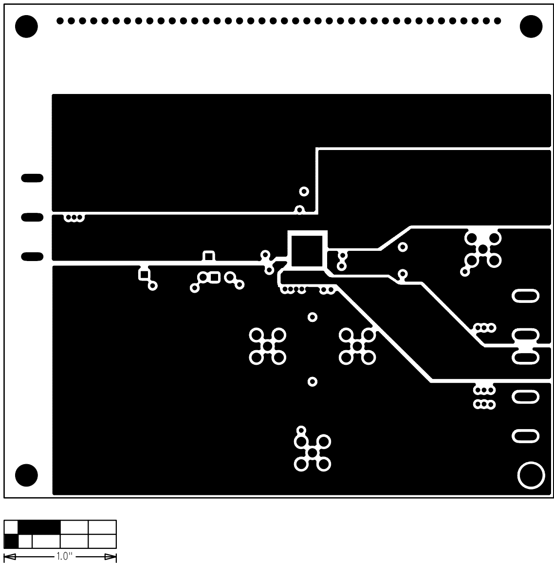
Figure 8. MAX5891/MAX5890/MAX5889 EV Kit PCB Layout—Power Planes (Layer 3)
