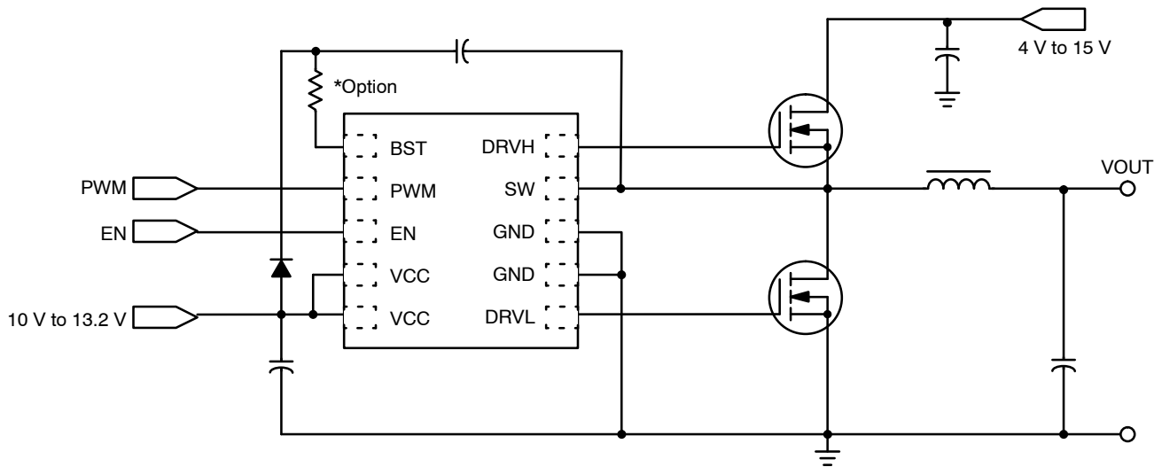
Figure 2. Typical Application
