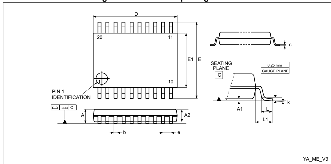
Figure 47. TSSOP20 package outline
