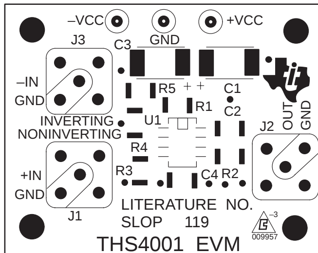
Figure 2–1. THS4001 EVM Component Placement Silkscreen and Solder Pads
