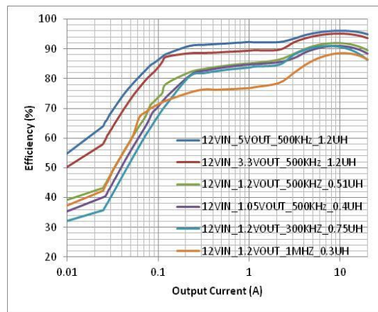
Figure 11. Efficiency vs. Load Current with V_{IN}=12\text{ V}
