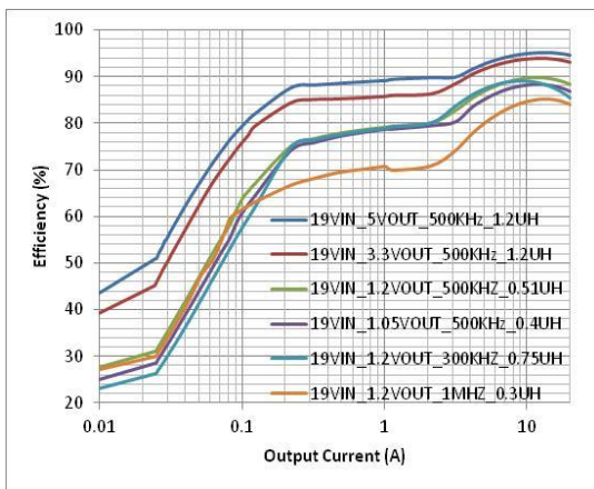
Figure 10. Efficiency vs. Load Current with V_{IN}=19\text{ V}
