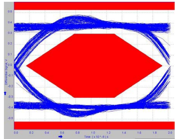
Figure 6. Audio Switch Near End Eye Diagram ( V_{CC} = 3.6 V, IN1 = 1, IN2 = 0, Temp = 25°C)
