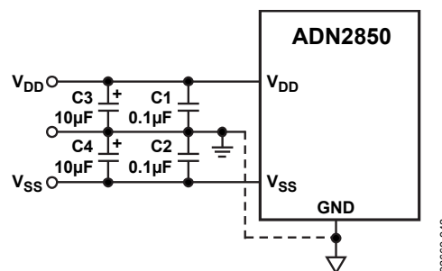
Figure 30. Power Supply Bypassing
