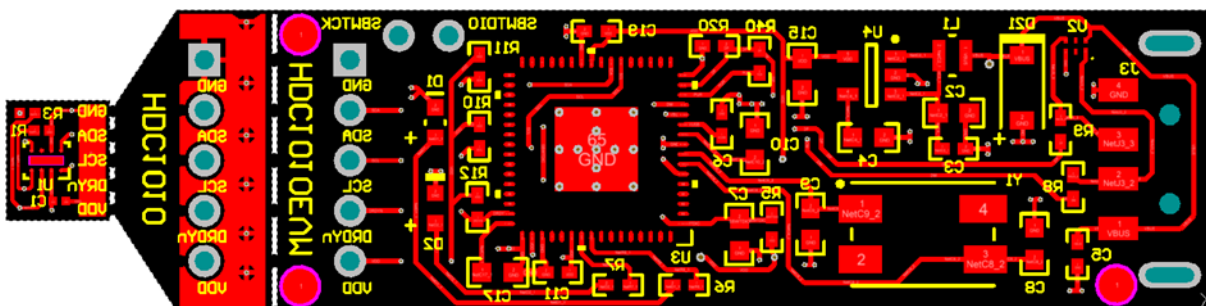
Figure 55. Top Layer Routing
