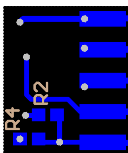
Figure 4. HDC1010EVM: Layout Resistors for I2C Address Setting - Bottom
