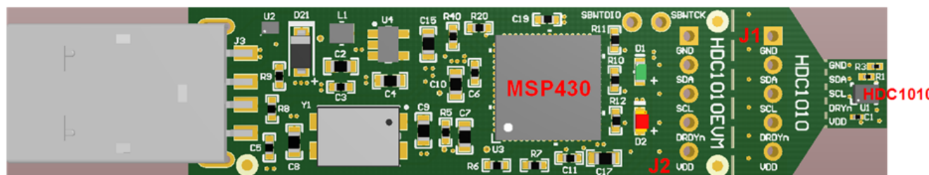
Figure 1. HDC1010EVM
