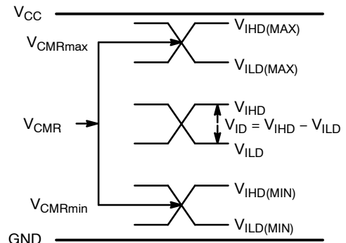
Figure 25. V_{CMR} Diagram
