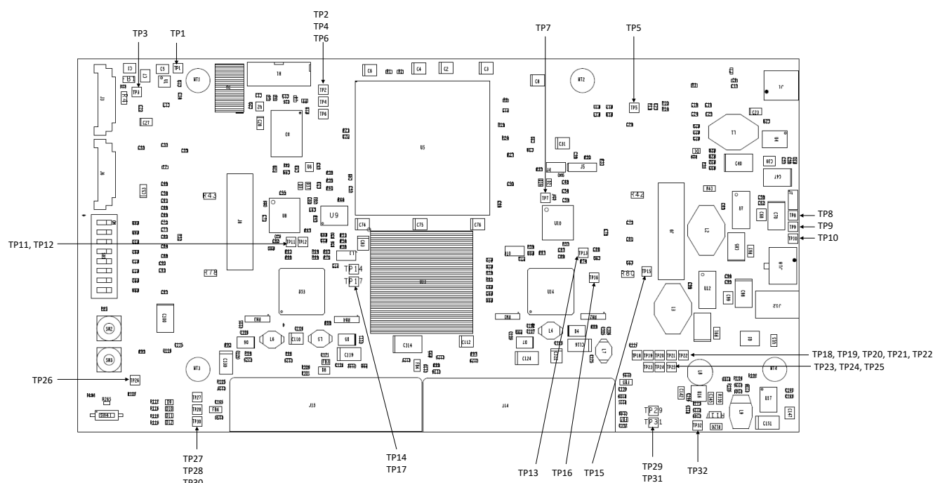
Figure 2-6. DLPLCRC410EVM Test Point Locations
