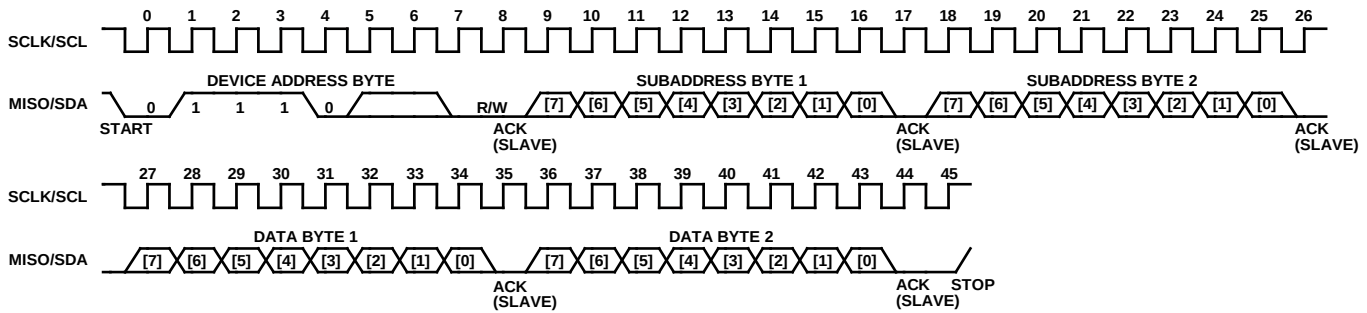
Figure 25. I²C Slave Single Word Write Operation (Two Bytes)
