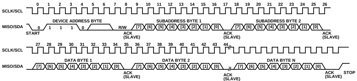
Figure 26. I²C Slave Burst Mode Write Operation (N Bytes)
