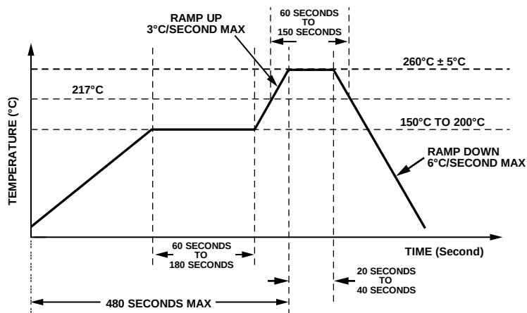
Figure 91. Soldering Profile
