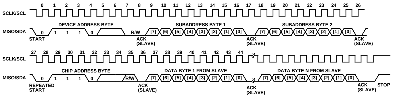
Figure 27. I²C Slave Burst Mode Read Operation (N Bytes)
