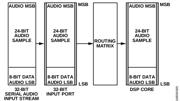
Figure 40. 32-Bit Serial Input Example
