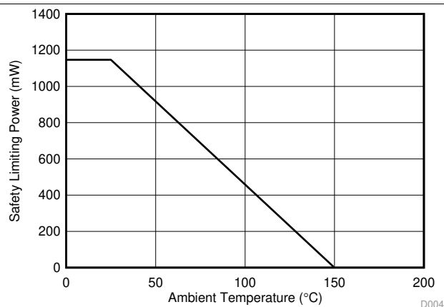
Figure 4. Thermal Derating Curve for Safety Limiting Power for DWW-16 Package
