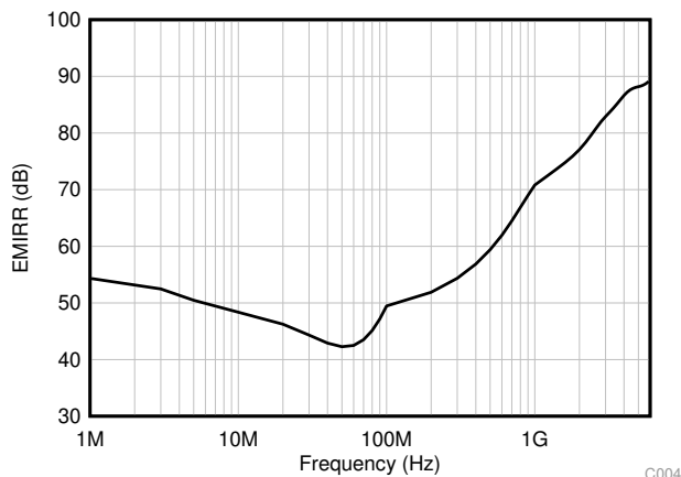
Figure 50. EMIRR Testing
