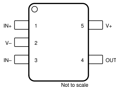
OPA990 DCK Package 5-Pin SC70 Top View
