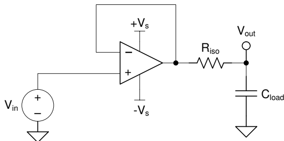
Figure 54. Extending Capacitive Load Drive With the OPA990
