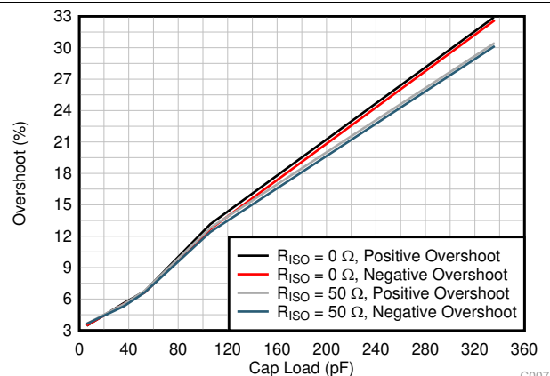
Figure 53. Small-Signal Overshoot vs Capacitive Load (10-mV Output Step, G = -1 )
