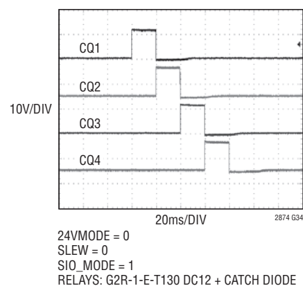
Driving 12V Relay Coils
