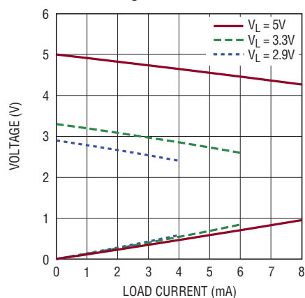
SDO Voltage vs Load Current
