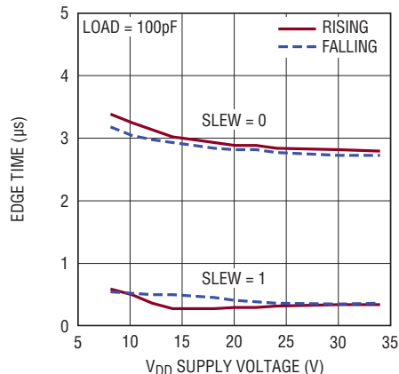
CQ Driver Edge Time vs Supply Voltage
