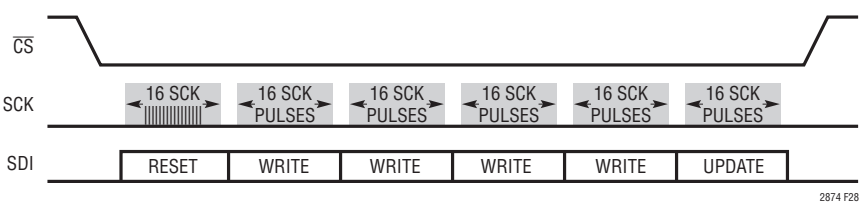
Figure 28. Continuous Transfer Capability
