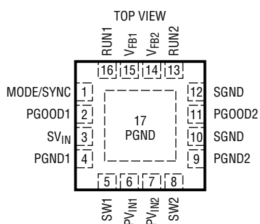
UD PACKAGE 16-LEAD (3mm × 3mm) PLASTIC QFN T_{JMAX} = 125^{\circ}C , \theta_{JA} = 68^{\circ}C/W , \theta_{JC} = 7.5^{\circ}C/W EXPOSED PAD (PIN 17) IS PGND, MUST BE SOLDERED TO PCB
