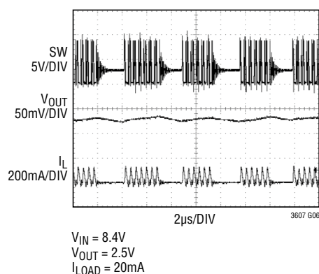
Pulse-Skipping Mode
