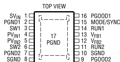
MSE PACKAGE 16-LEAD PLASTIC MSOP T_{JMAX} = 125^{\circ}C , \theta_{JA} = 37^{\circ}C/W , \theta_{JC} = 10^{\circ}C/W EXPOSED PAD (PIN 17) IS PGND, MUST BE SOLDERED TO PCB
