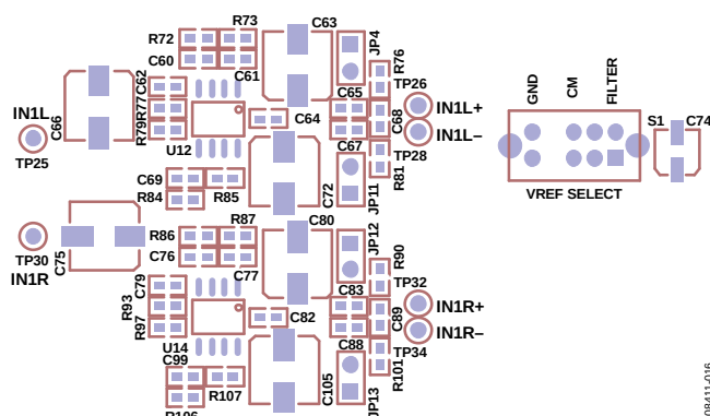
Figure 16. VREF Selection and DC Coupling Jumpers
