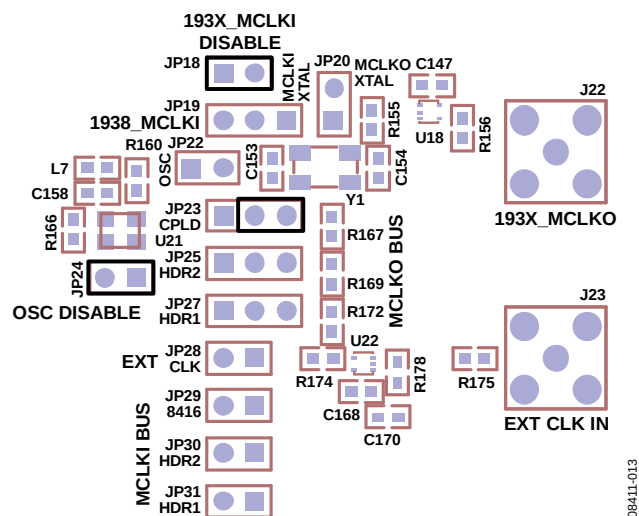
Figure 13. LRCLK Is the Master Clock Using the PLL; MCLKI Is Disabled, and CPLD Is Slave to the MCLKO Port
