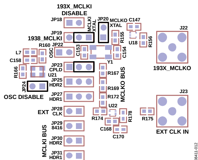
Figure 12. Passive Crystal; the AD1939 Is Master and the CPLD Is Slave from the MCLKO Port
