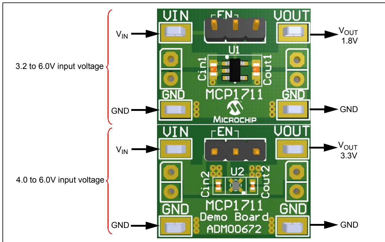
FIGURE 2-1: MCP1711 Demo Board - Powering Sequence.
