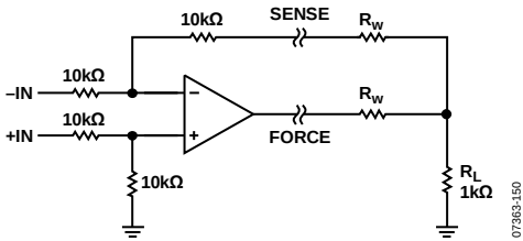
Figure 52. Connecting Both the Output and Feedback at the Load Minimizes Error Due to Wire Resistance
