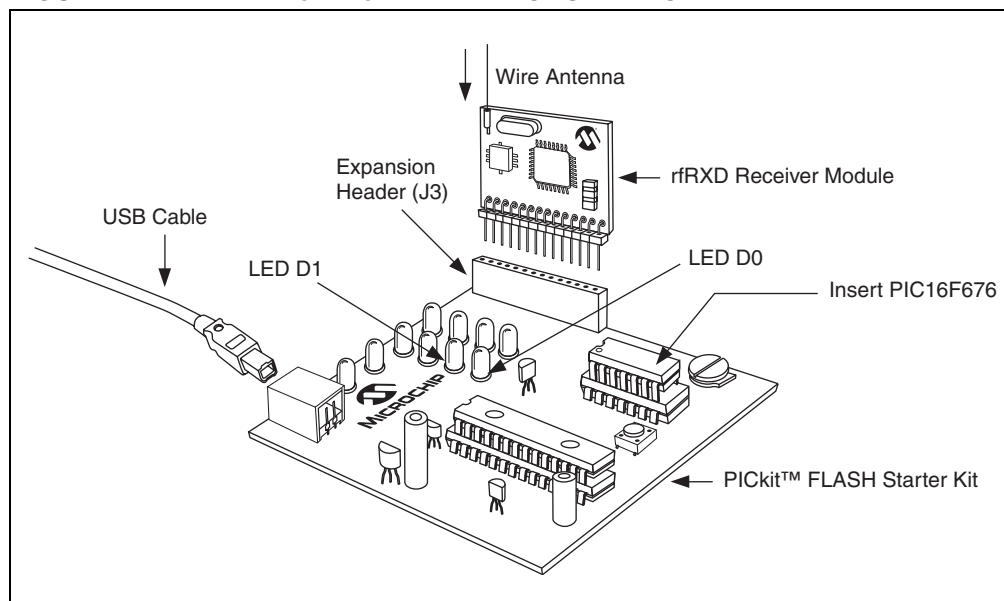
FIGURE 1-1: rfPIC RECEIVER DEMONSTRATION
