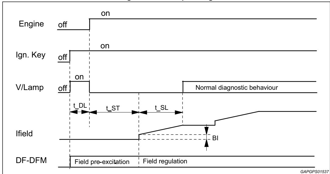
Figure 5. Start-up timing
