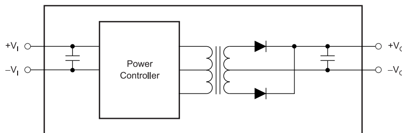
Figure 20. Single-Output Block Diagram
