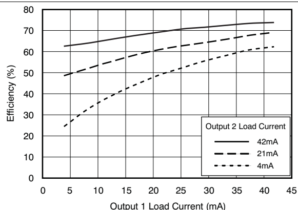
Figure 8. DCH010512D Efficiency
