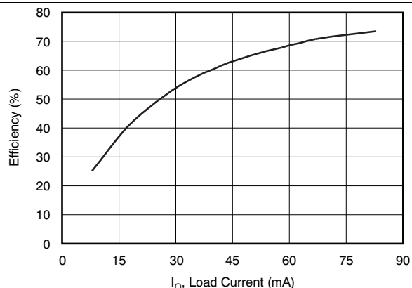
Figure 7. DCH010512S Efficiency
