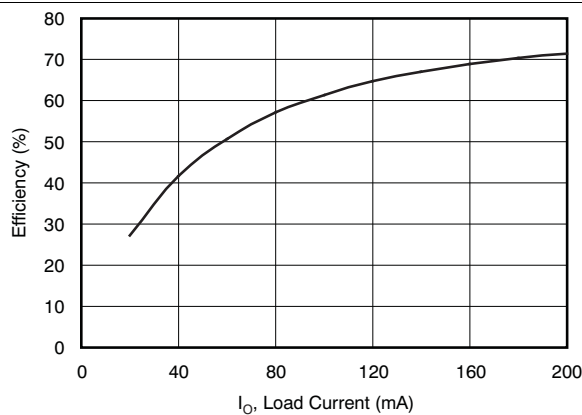
Figure 28. DCH010505S Efficiency
