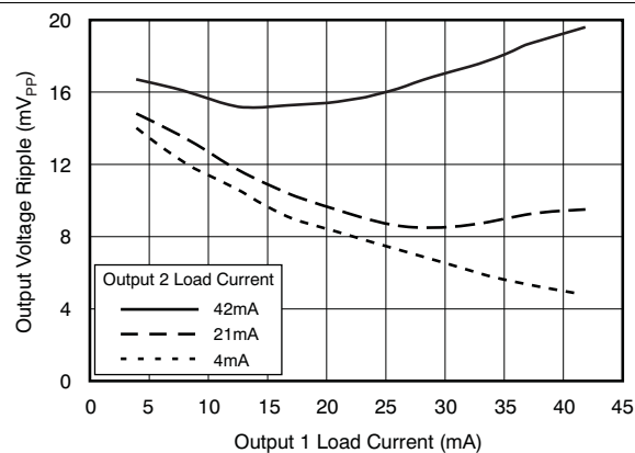
Figure 12. DCH010512D Ripple Voltage
