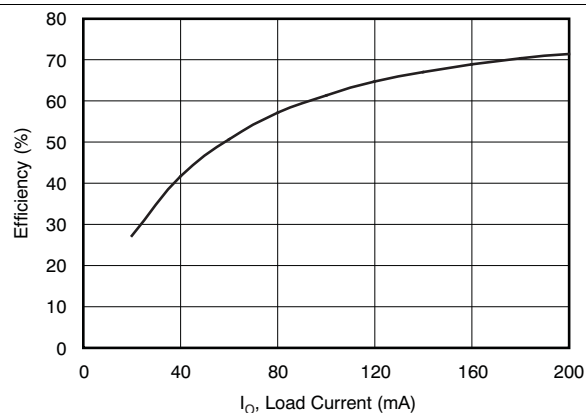
Figure 1. DCH010505S Efficiency
