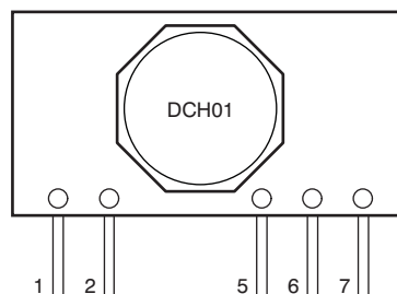
EDJ Package 7-Pin SIP (Dual) Top View
