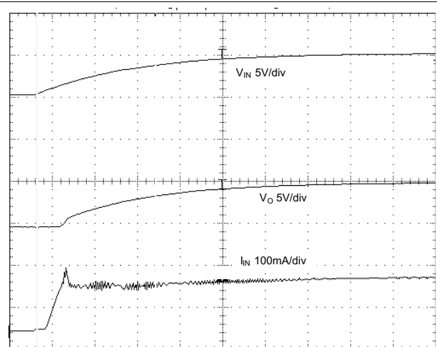
Figure 29. DCH010505S Start-up Waveforms
