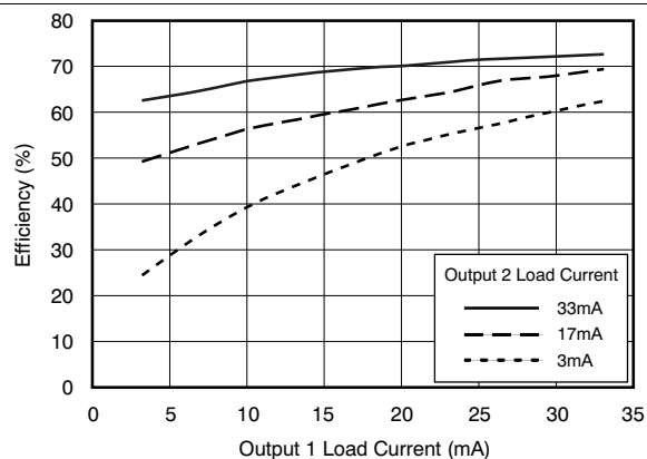
Figure 14. DCH010515D Efficiency
