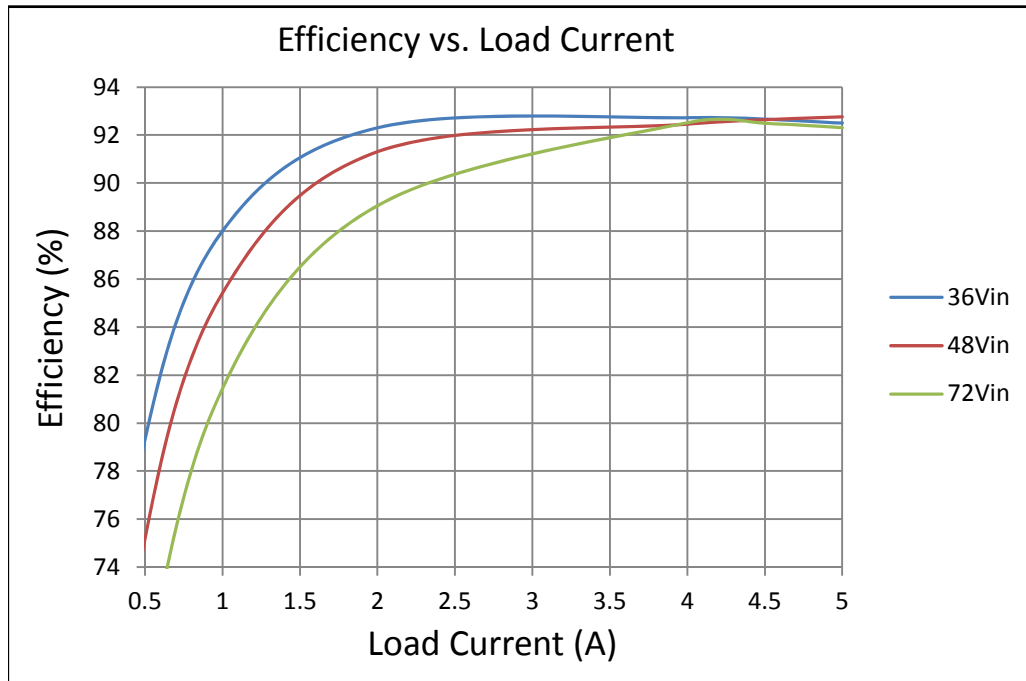
Figure 3. Efficiency
