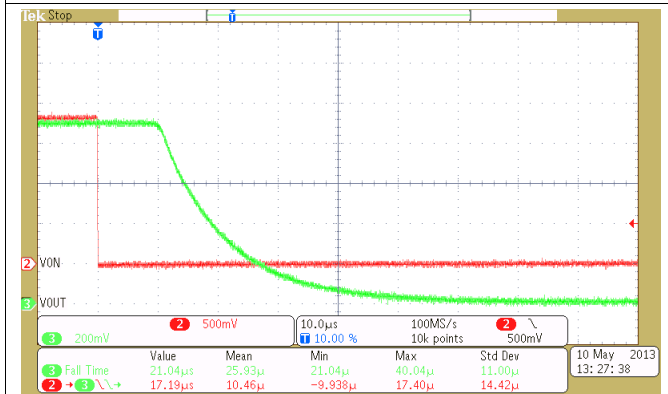
Figure 21. Turnoff Response ( C_{IN} = 10 \mu F , C_L = 1 \mu F , R_L = 10 \Omega , V_{IN} = 0.9 V , T_A = 25^\circ C )
