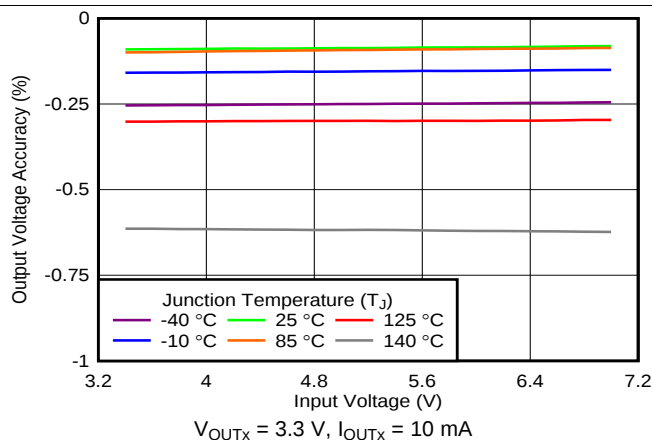
Figure 28. Line Regulation
