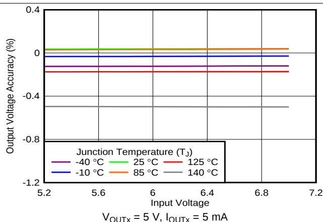
Figure 30. Line Regulation
