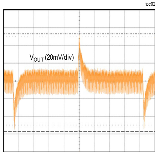
TIME: 100μs/div CONDITIONS: I OUT = 15A to 22.5A STEP at 1A/μs
