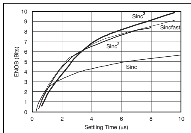
Figure 28. Measured ENOB vs Settling Time
