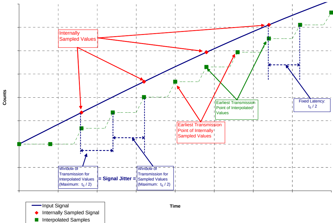
Figure 23. Data Interpolation Example
