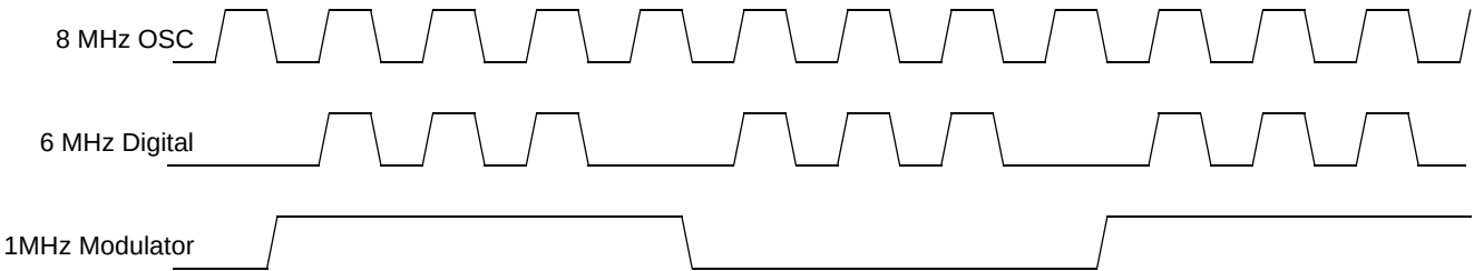
Figure 13. Clock Generation
