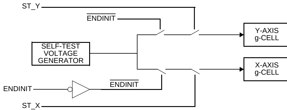
Figure 10. Self-test Interface
