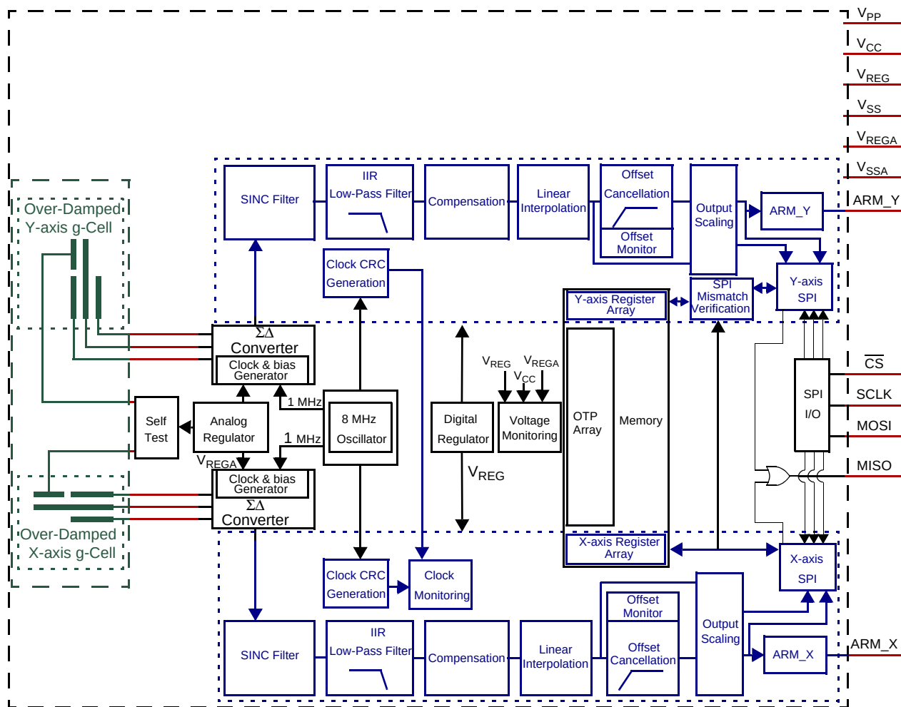
Figure 4. Block Diagram
