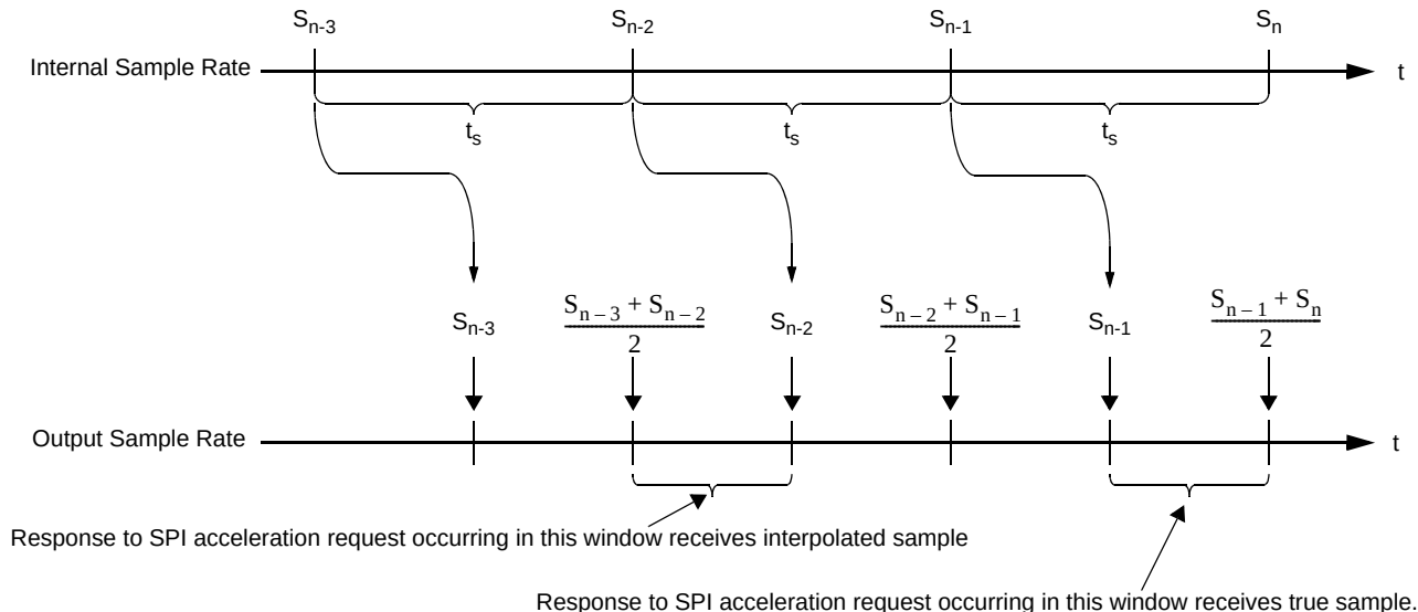
Figure 22. Data Interpolation Timing
