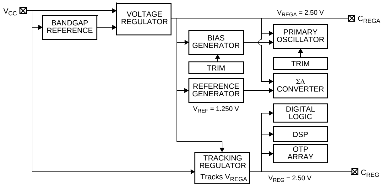
Figure 8. Power Supply
