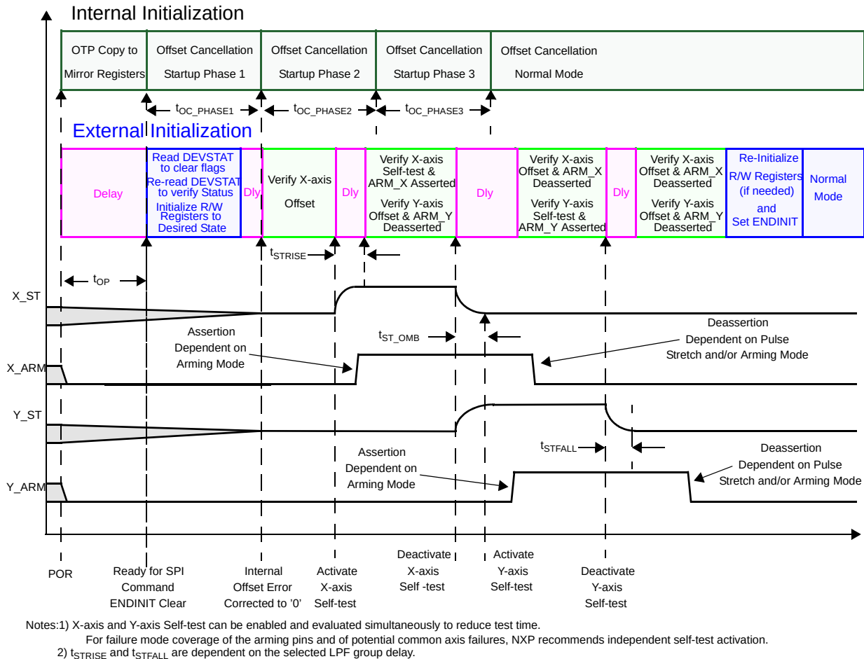
Figure 32. Initialization Process
