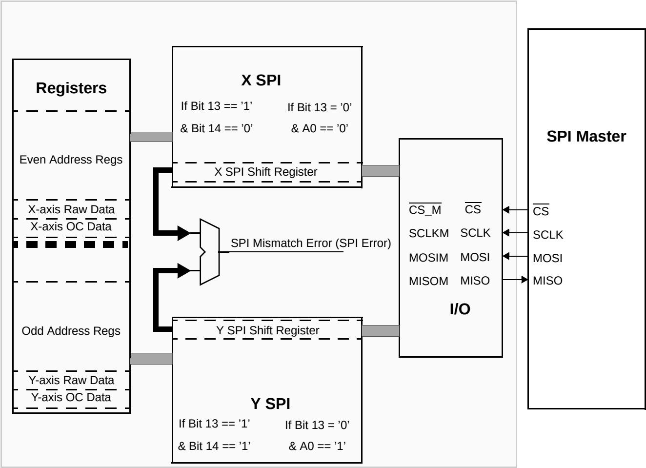
Figure 31. SPI Diagram
