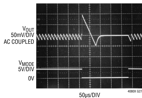
Output Voltage Transient Step Response (Burst Mode)
