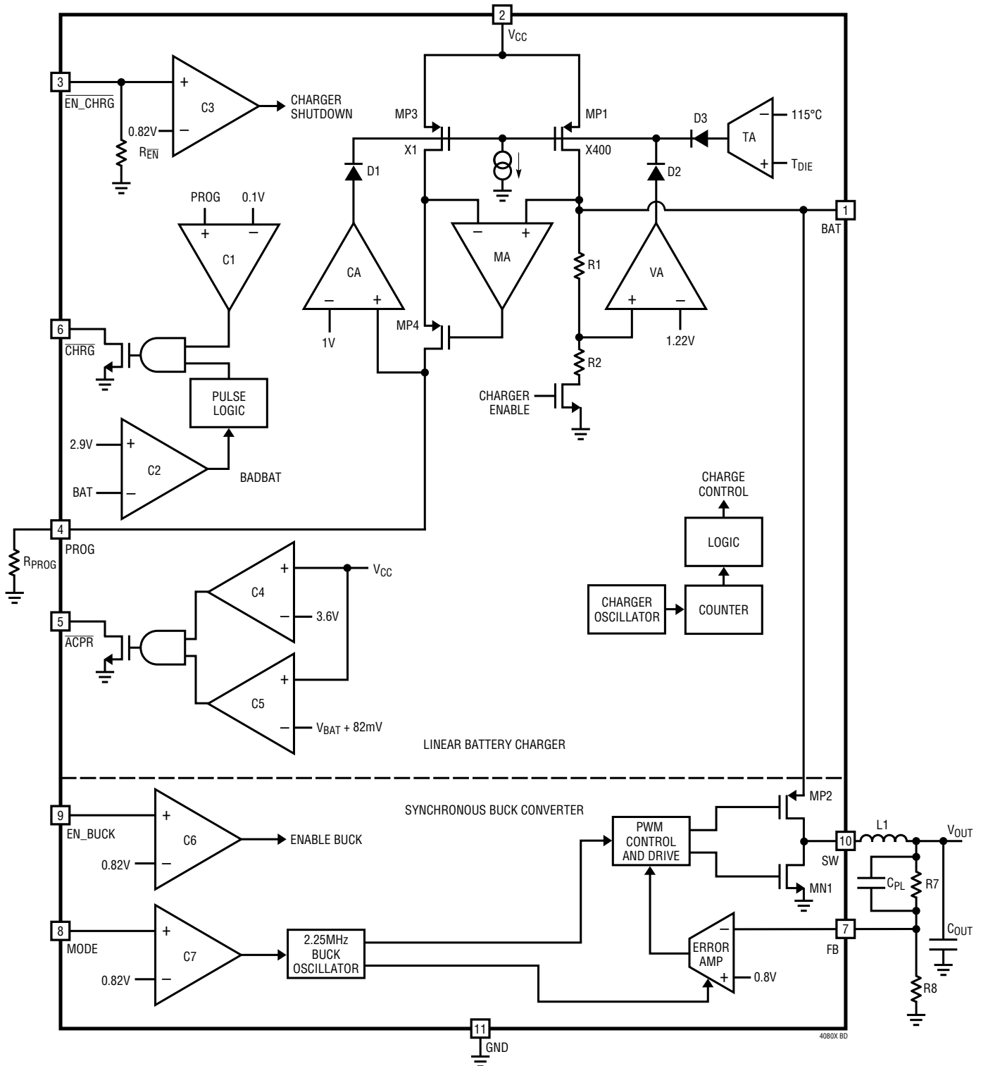
Figure 1. LTC4080X Block Diagram
