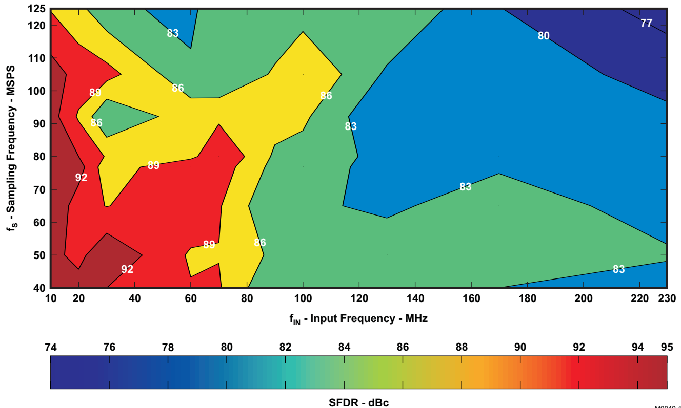
Figure 28. SFDR Contour
