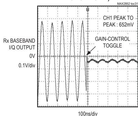
Rx BASEBAND VGA SETTLING RESPONSE (+30dB BASEBAND VGA GAIN STEP)
