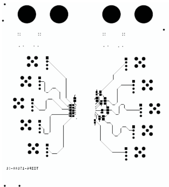
Figure 11. Signal Traces On Bottom Layer
