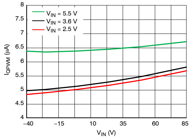
Figure 6. PWM Quiescent Current vs. Temperature (EN = High, Open Loop, V_{OUT} = 1.8\text{ V} , V_{IN} = 3.6\text{ V} )
