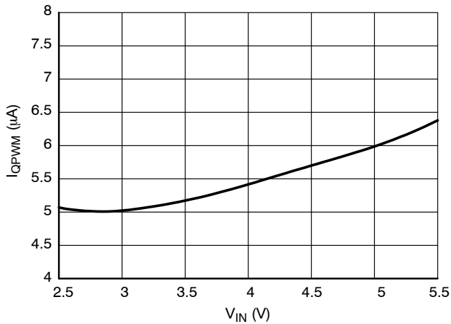
Figure 5. PWM Quiescent Current vs. Input Voltage (EN = High, Open Loop, V_{OUT} = 1.8\text{ V} , T_A = 25^\circ\text{C} )
