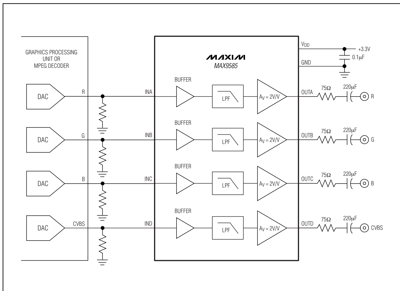
Figure 1. AC-Coupled Outputs
