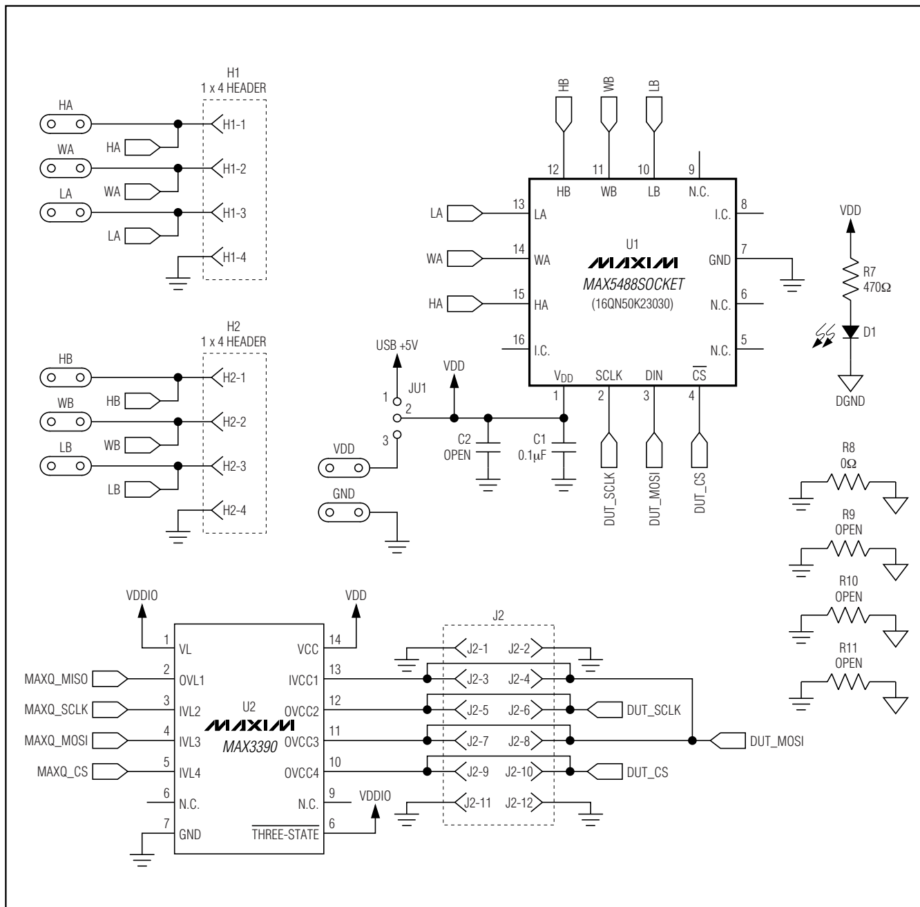
Figure 2a. MAX5488 EV Kit Schematic (Sheet 1 of 3)
