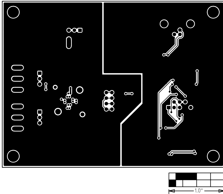
Figure 5. MAX5488 EV Kit PCB Layout—Solder Side
