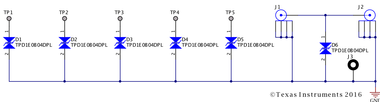
Figure 4. TPD1E0B04EVM Schematic
