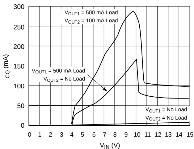
Figure 12. Quiescent Current ( I_{CQ} ) vs. V_{IN} Over R_{LOAD}
