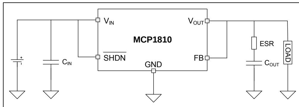
FIGURE 1-1: MCP1810 Typical Application
