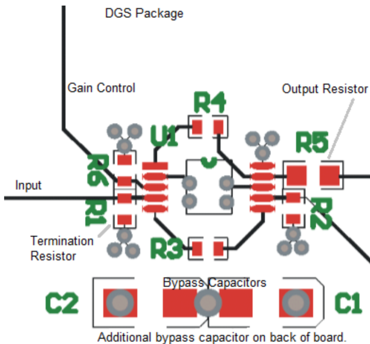
Figure 78. Layout Recommendation
