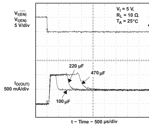
Figure 24. Inrush Current With Different Load Capacitance
