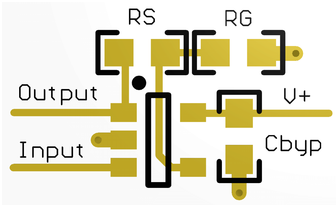
Figure 55. Layout Recommendation
