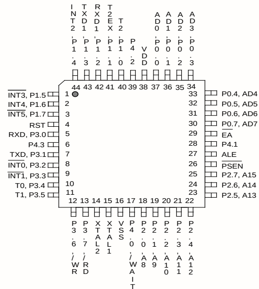
44-Pin QFP
