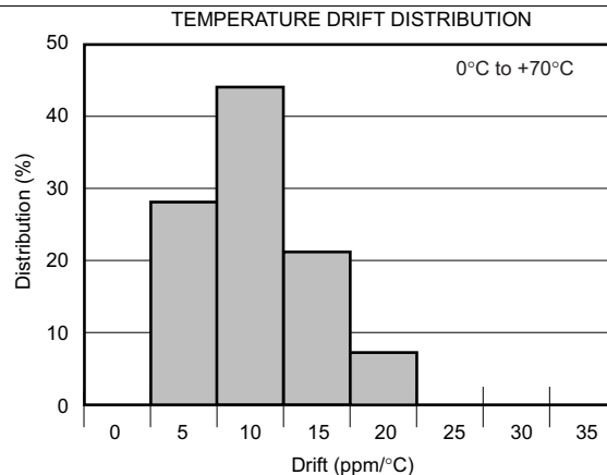
Figure 8. Temperature Drift Distribution
