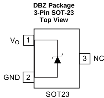
Pin Functions
