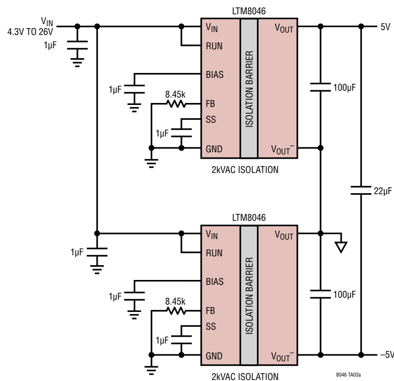
Use Two LTM8046 Flyback Converters to Generate ±5V
