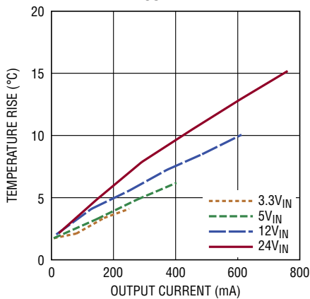
Temperature Rise vs Output Current 2.5V OUT
