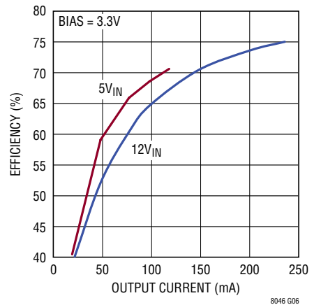
12V OUT Efficiency vs Output Current
