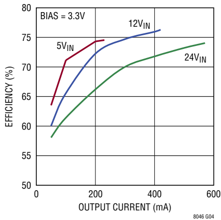
5V OUT Efficiency vs Output Current
