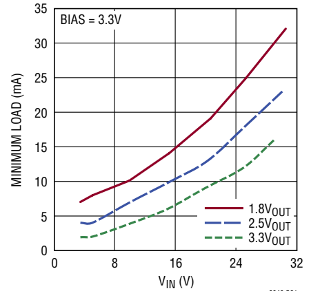
Minimum Load vs V_{IN}
