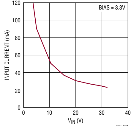
Input Current vs V_{IN} Output Shorted
