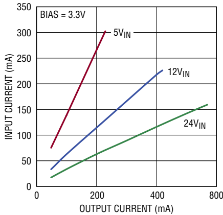
5V OUT Input Current vs Output Current
