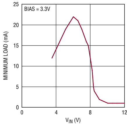
12V OUT Minimum Load vs V_{IN}
