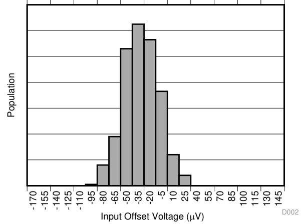
Figure 2. Input Offset Voltage Production Distribution A2
