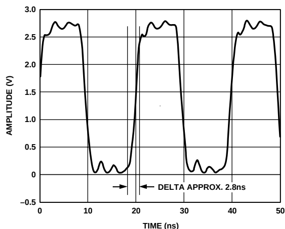
Figure 53. DATACLK Driver Capability into 330\ \Omega at 50\text{ MHz}
