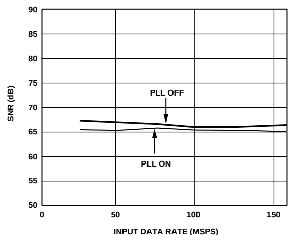
Figure 22. SNR vs. Data Rate for f_{OUT} = 5 \text{ MHz}
