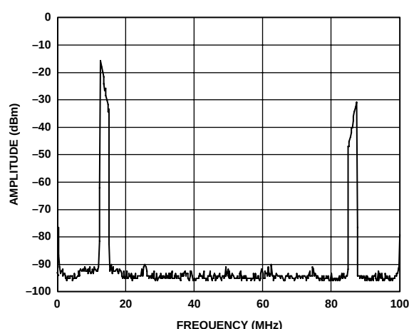
Figure 95. AD9775 Real DAC Output of Complex Input Signal Near Baseband (Positive Frequencies Only), Interpolation = 8x, Complex Modulation in AD9775 = +f_{DAC}/8
