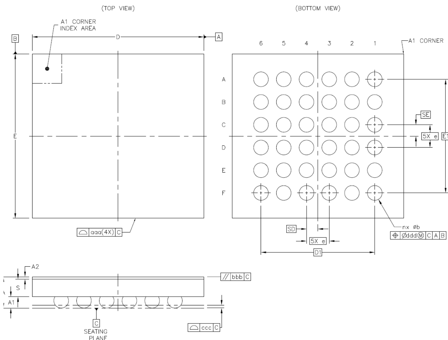
Figure 6.1. CSP81
