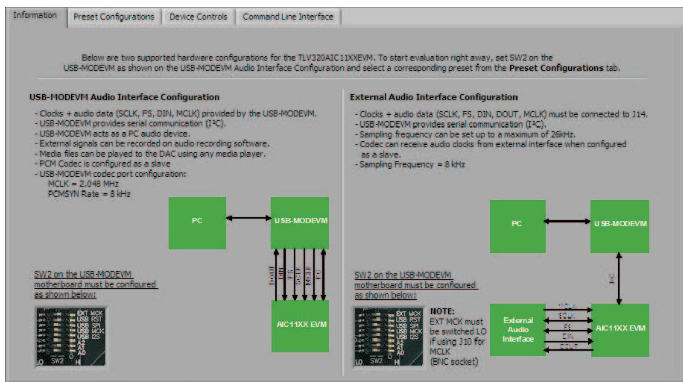
Figure 4. Information Tab
