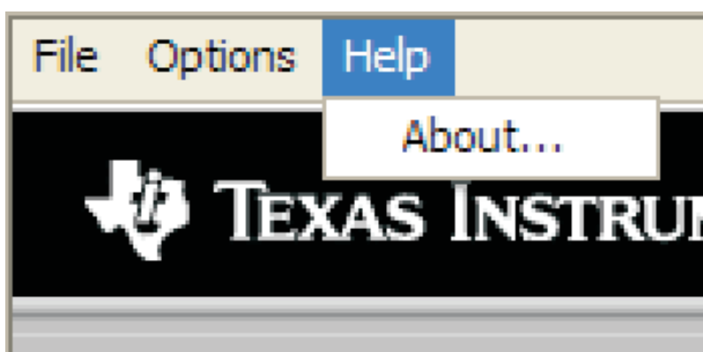
Figure 10. Help
