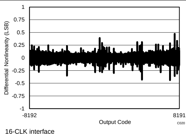
Figure 44. Typical DNL
