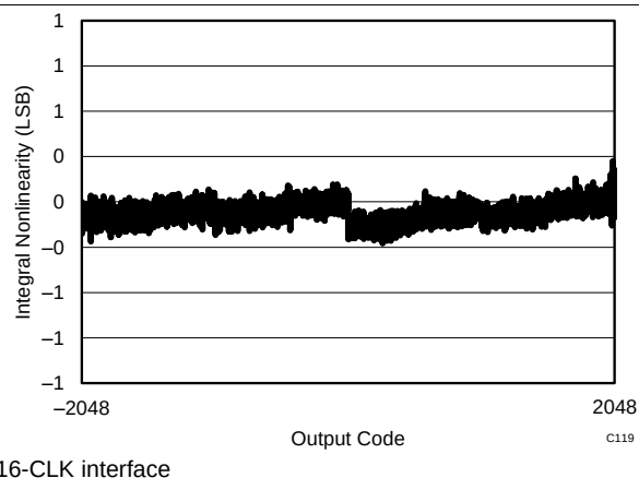
Figure 73. Typical INL
