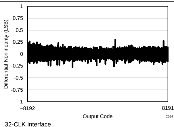
Figure 46. Typical DNL
