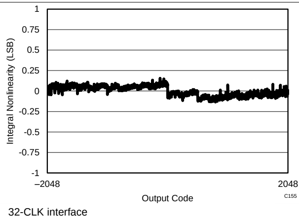
Figure 75. Typical INL
