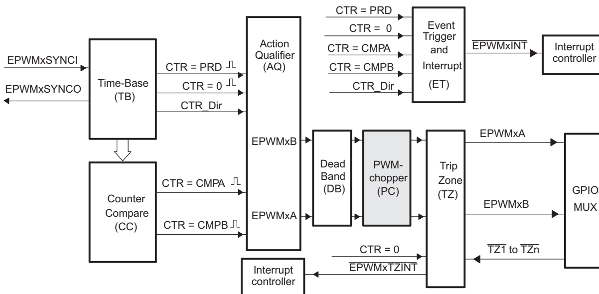
Figure 16-31. PWM-Chopper Submodule
