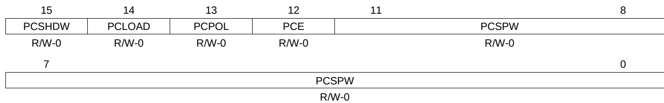
Figure 17-35. eQEP Position-Compare Control Register (QPOSCTL)
