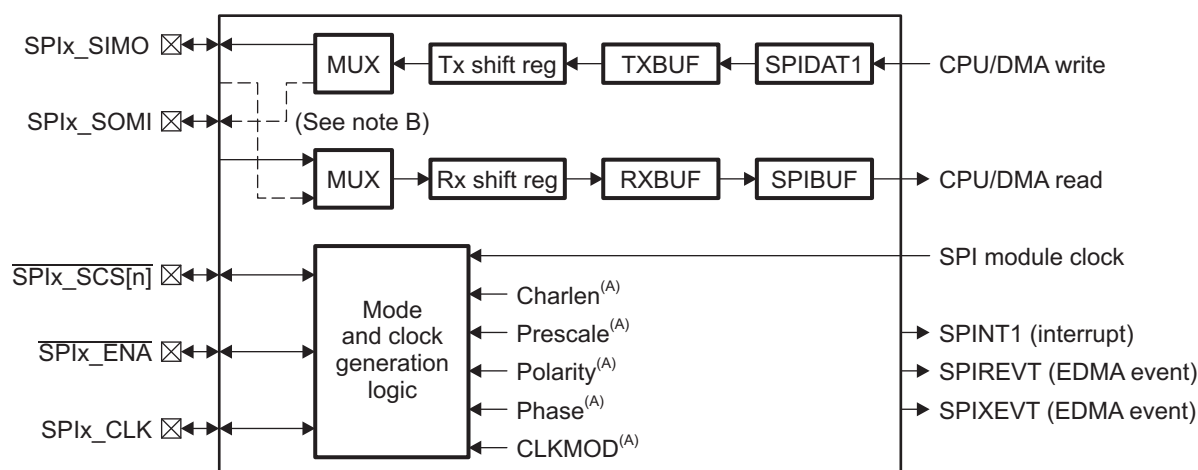
Figure 29-1. SPI Block Diagram
