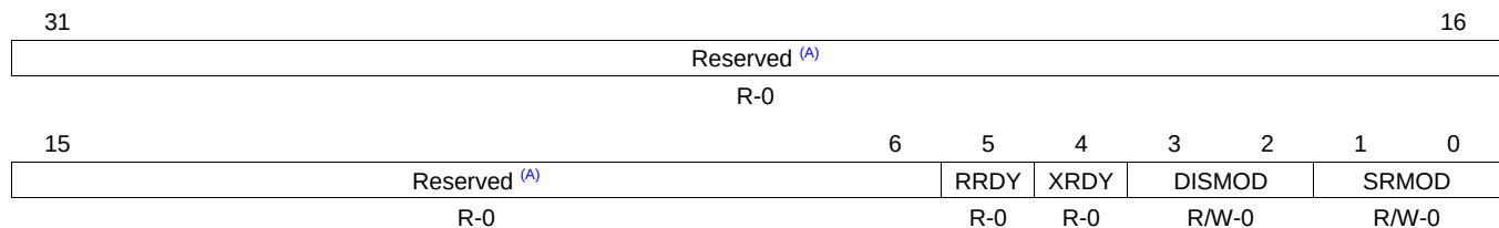
Figure 26-70. Serializer Control Registers (SRCTL n )
