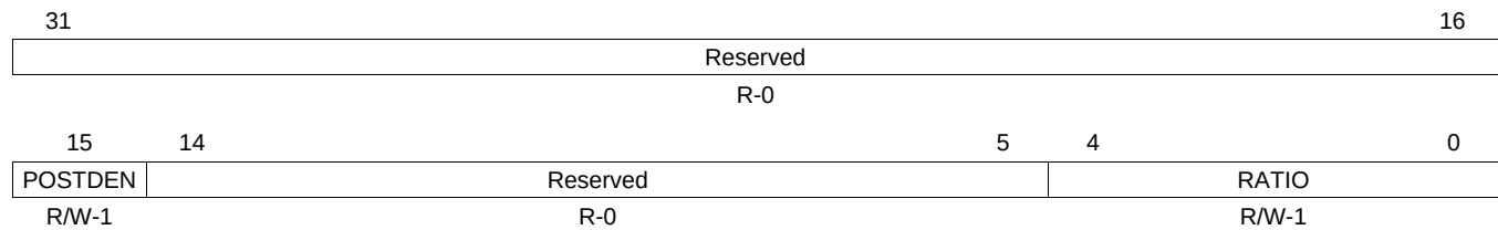
Figure 8-16. PLL Post-Divider Control Register (POSTDIV)
