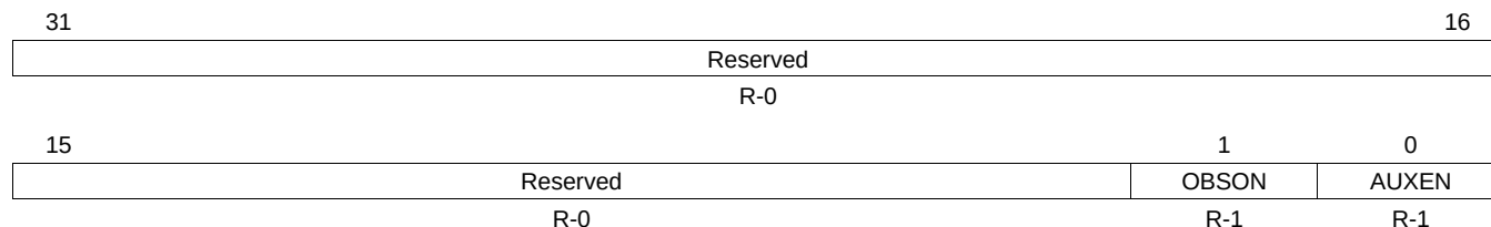
Figure 8-22. Clock Status Register (CKSTAT)
