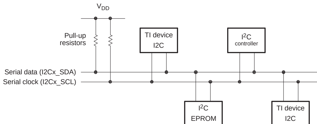
Figure 24-2. Multiple I2C Modules Connected
