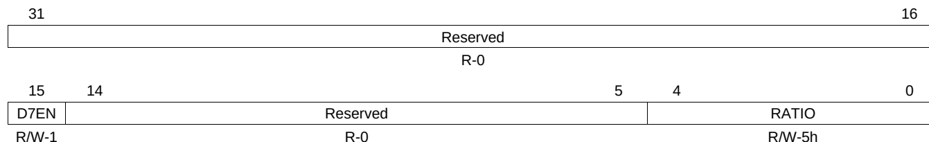
Figure 8-14. PLL Controller Divider 7 Register (PLLDIV7)
