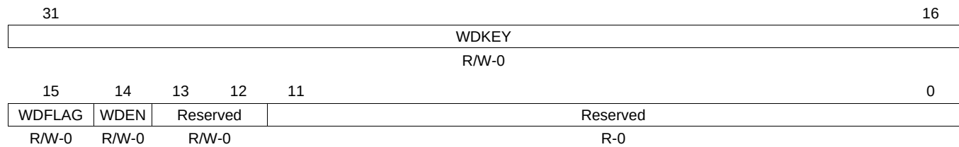
Figure 30-23. Watchdog Timer Control Register (WDTCR)
