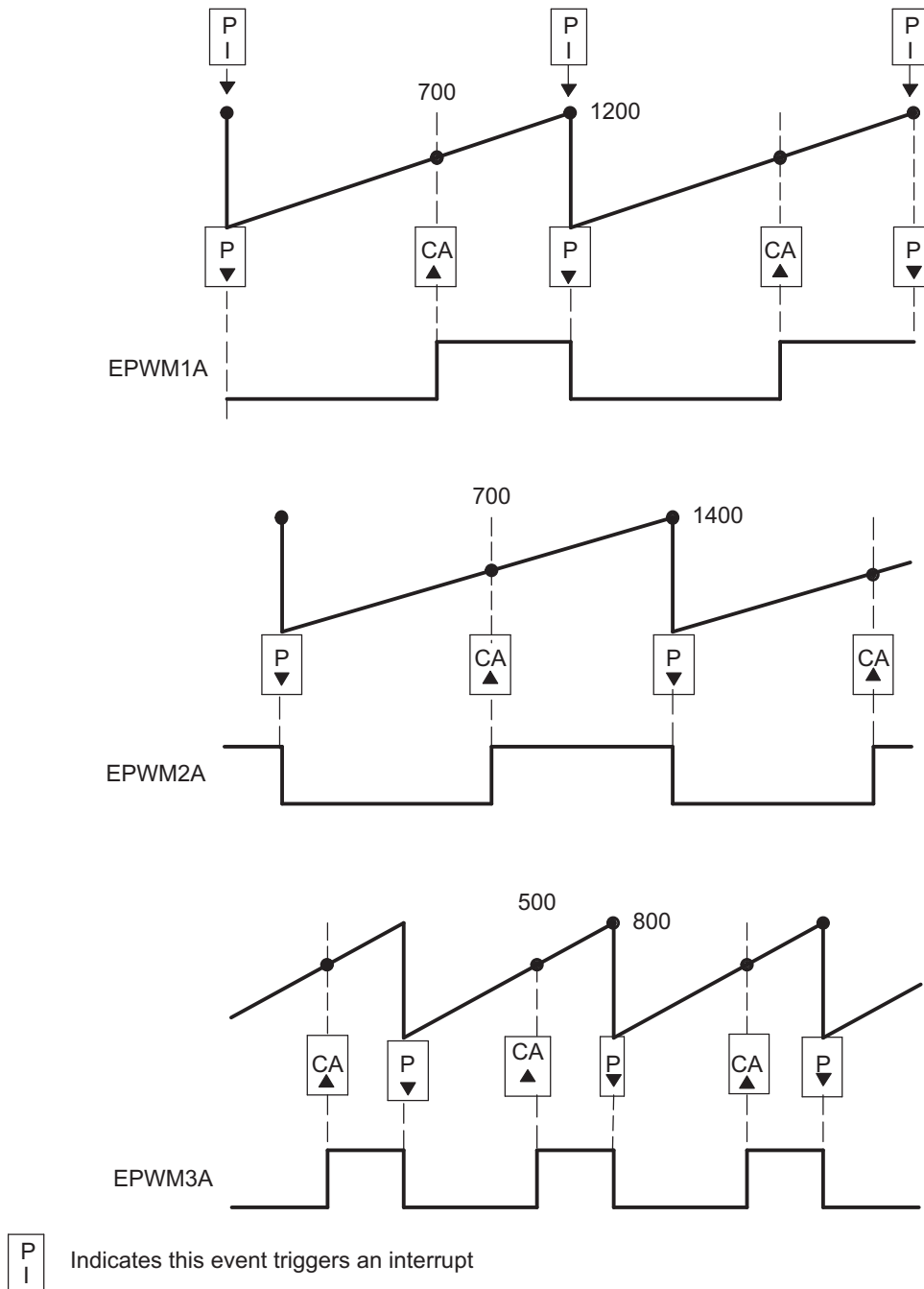
Figure 16-52. Buck Waveforms for Figure 16-51 (Note: Only three bucks shown here)
