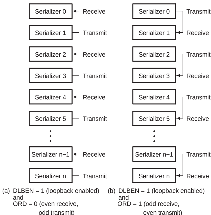
Figure 26-34. Serializers in Loopback Mode
