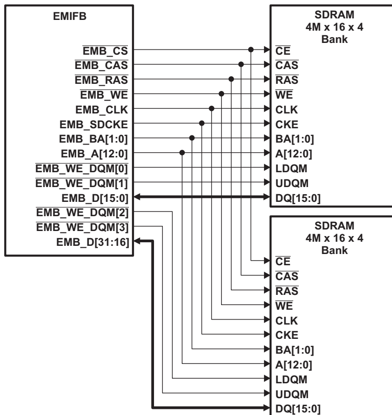
Figure 21-11. Connecting EMIFB Memory Controller for 32-bit Connection
