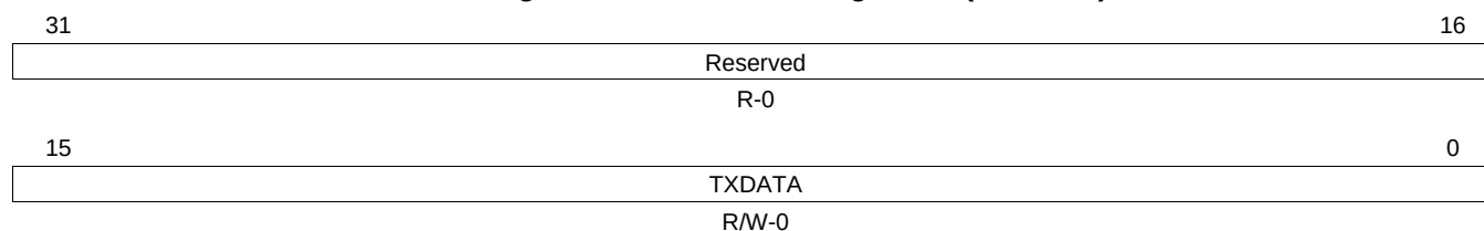
Figure 29-29. SPI Data Register 0 (SPIDAT0)
