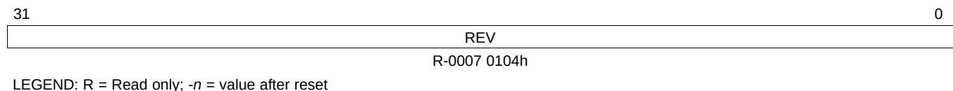
Figure 19-25. MDIO Revision ID Register (REVID)
