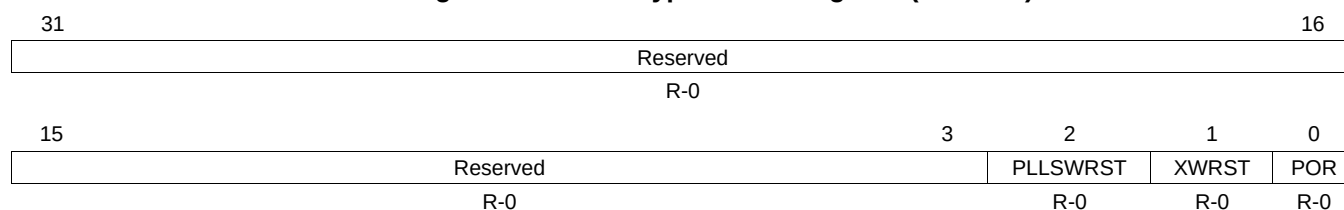
Figure 8-3. Reset Type Status Register (RSTYPE)
