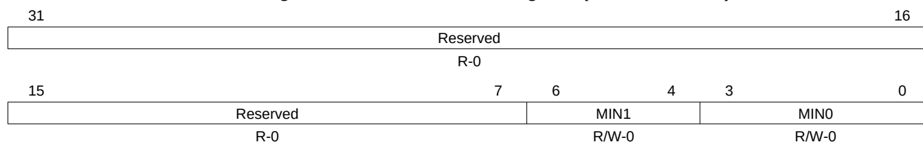
Figure 28-12. Alarm Minute Register (ALARMMINUTE)
