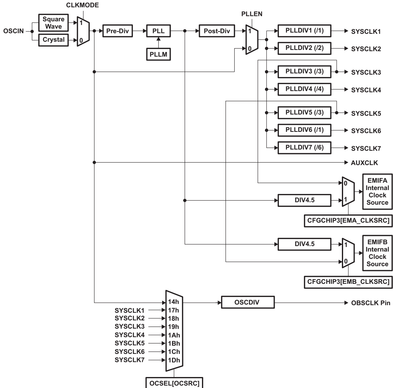
Figure 8-1. PLL0 Structure
