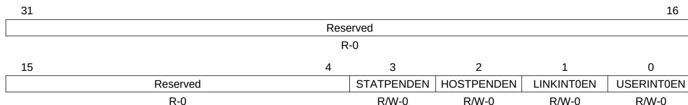
Figure 19-18. EMAC Control Module Interrupt Core 0-2 Miscellaneous Interrupt Enable Register (CnMISCEN)
