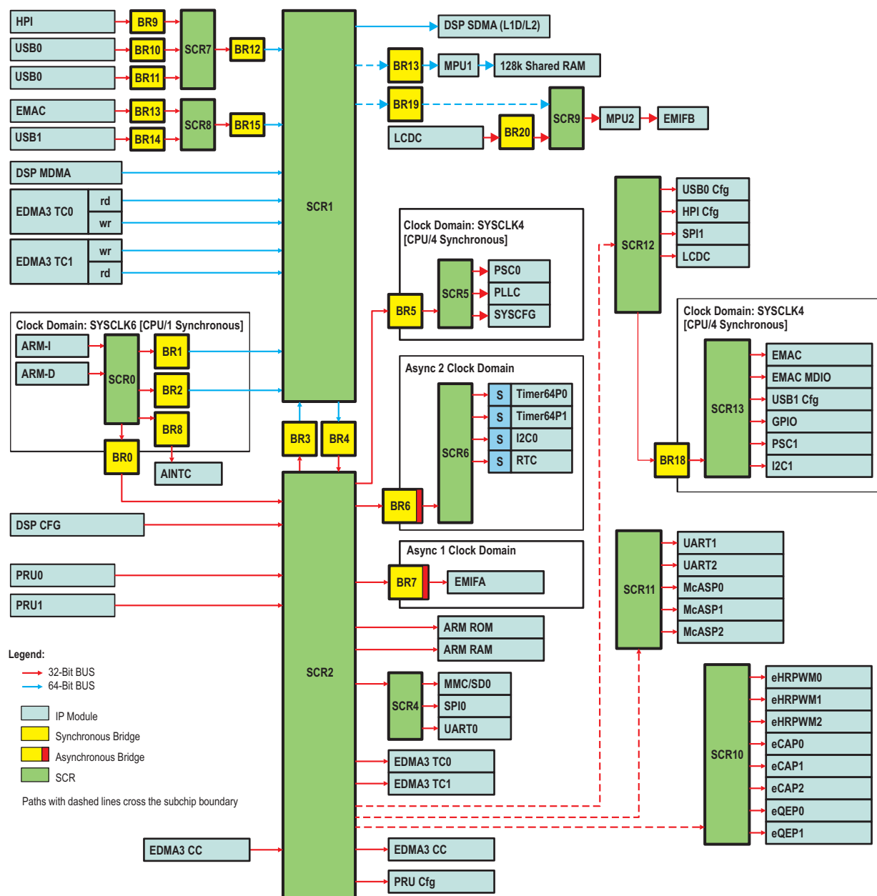
Figure 4-1. System Interconnect Block Diagram
