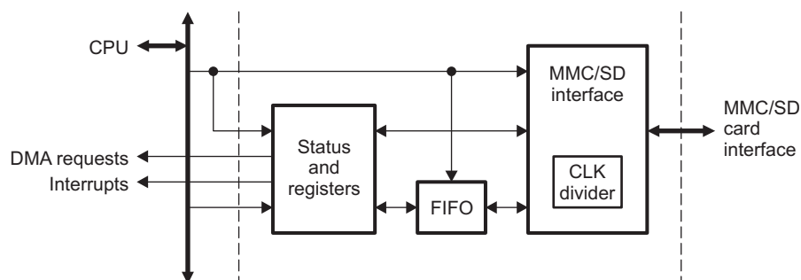
Figure 27-1. MMC/SD Card Controller Block Diagram
