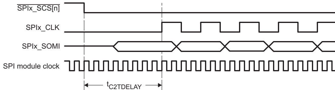
Figure 29-34. Example: t_{\text{C2DELAY}} = 8 SPI Module Clock Cycles
