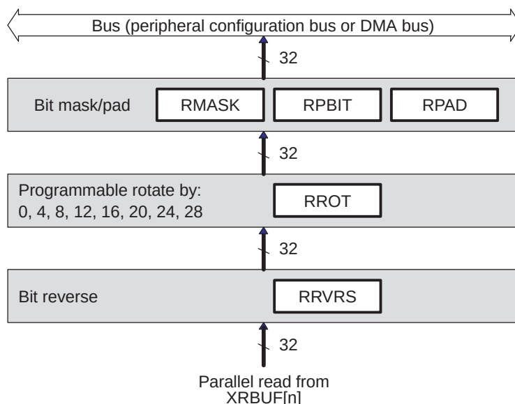
Figure 26-19. Receive Format Unit
