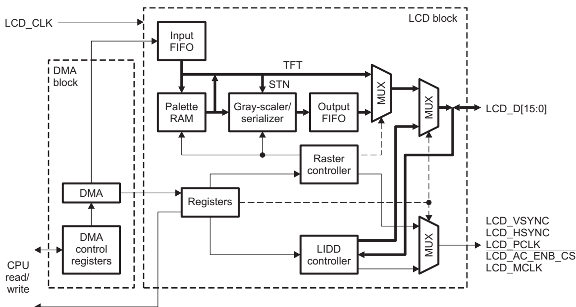
Figure 25-1. LCD Controller
