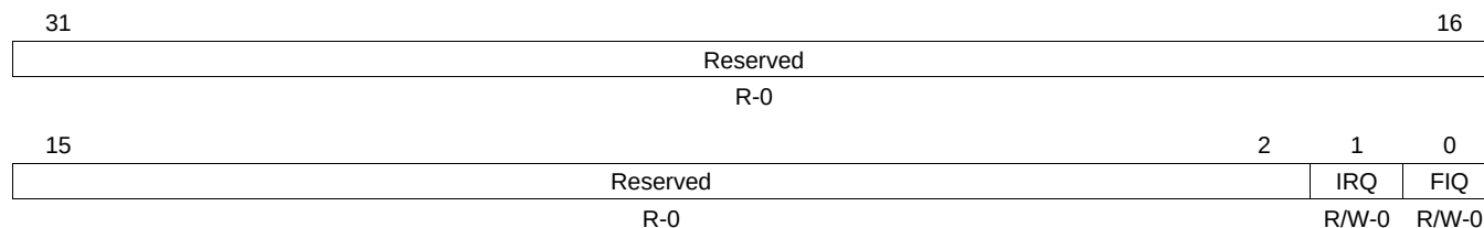
Figure 12-35. Host Interrupt Enable Register (HIER)
