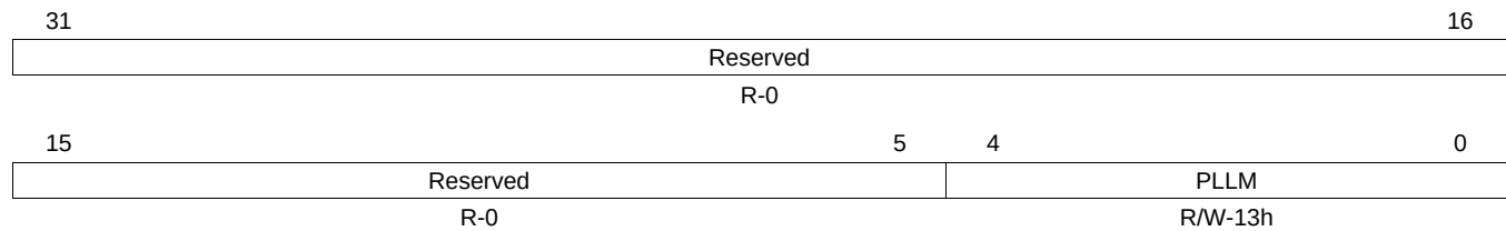
Figure 8-6. PLL Multiplier Control Register (PLLM)
