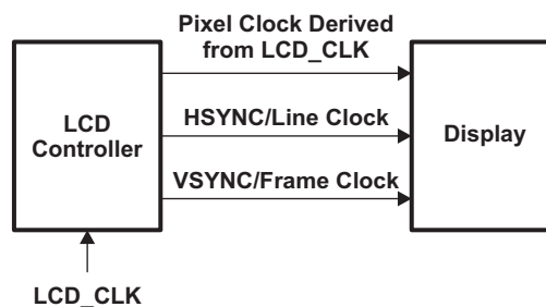
Figure 25-2. Input and Output Clocks
