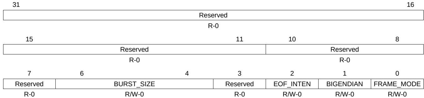
Figure 25-41. LCD DMA Control Register (LCDDMA_CTRL)
