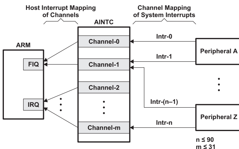
Figure 12-1. AINTC Interrupt Mapping
