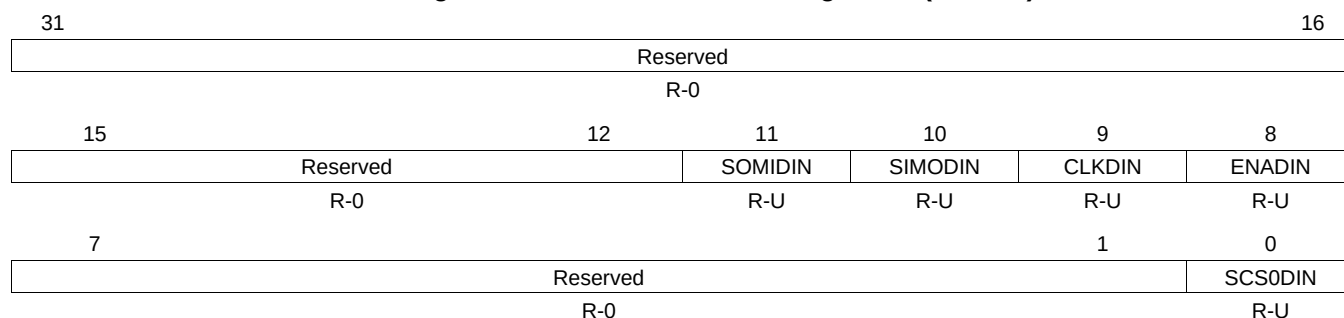
Figure 29-25. SPI Pin Control Register 2 (SPIPC2)
