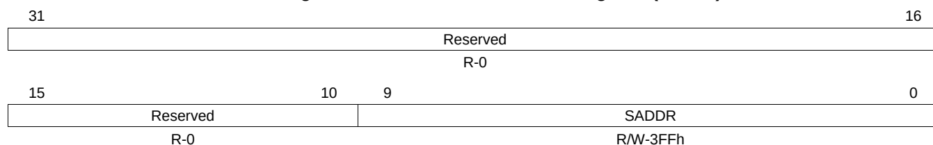
Figure 24-20. I2C Slave Address Register (ICSAR)
