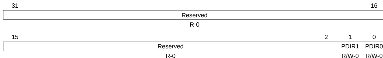
Figure 24-31. I2C Pin Direction Register (ICPDIR)
