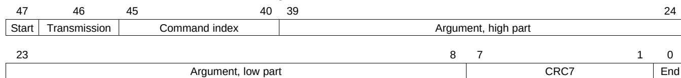
Figure 27-30. Command Format
