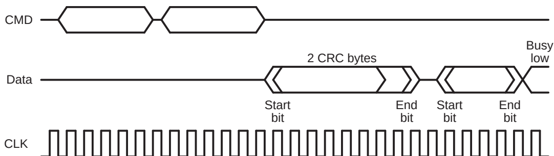
Figure 27-5. MMC/SD Mode Write Sequence Timing Diagram
