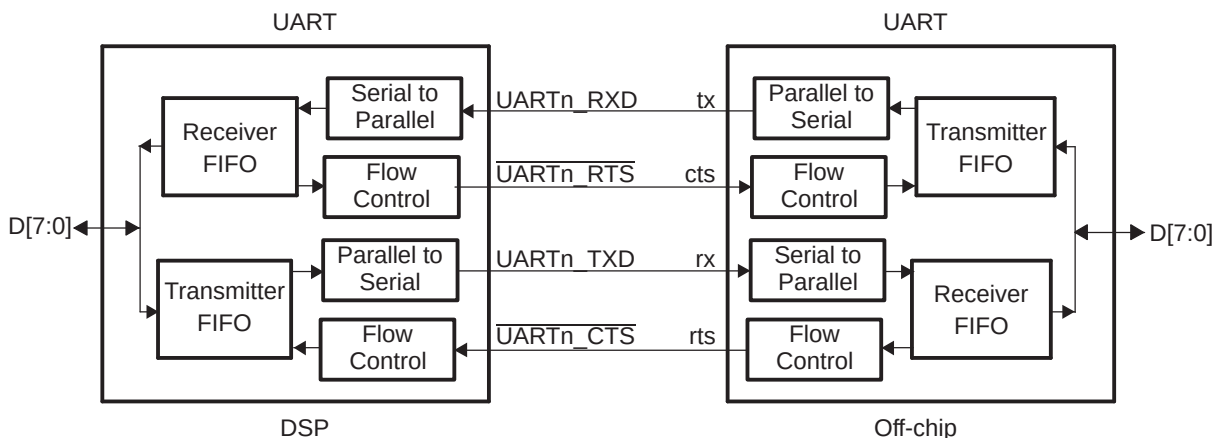
Figure 31-5. UART Interface Using Autoflow Diagram
