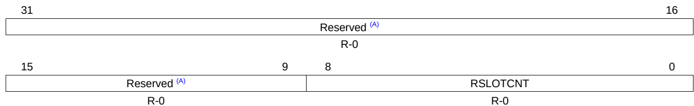
Figure 26-55. Current Receive TDM Time Slot Registers (RSL0T)
